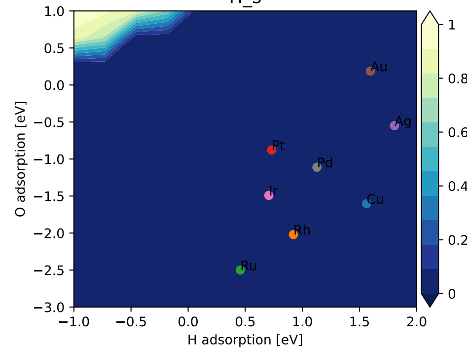
H_s
